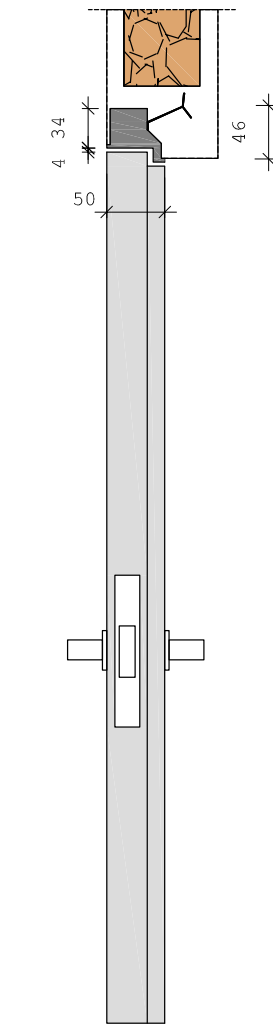
Pull opening
