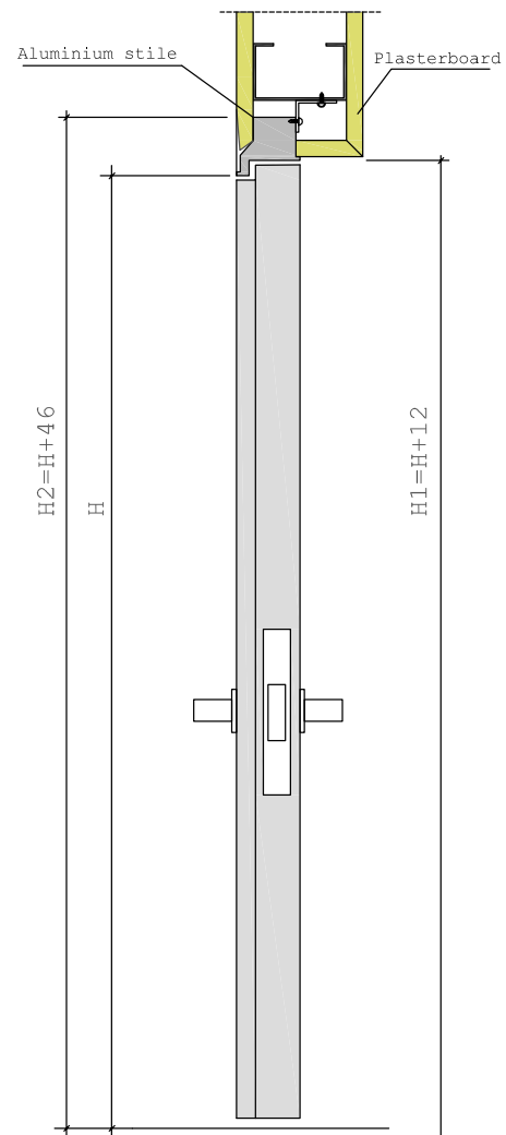
Push opening
